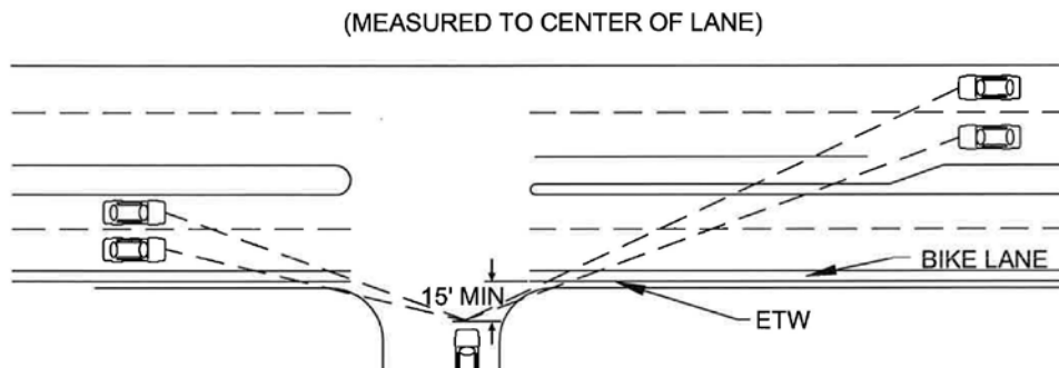
EXHIBIT 7-2 CORNER SIGHT DISTANCE:
